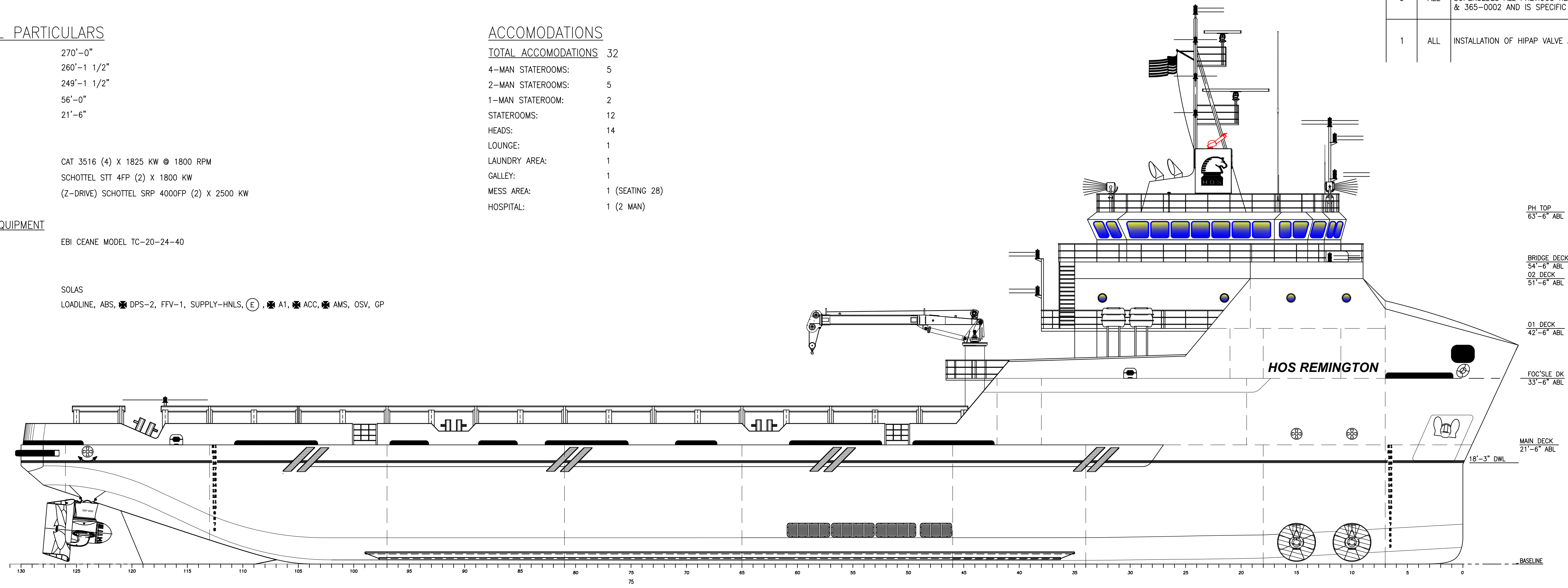
OUTBOARD PROFILE
