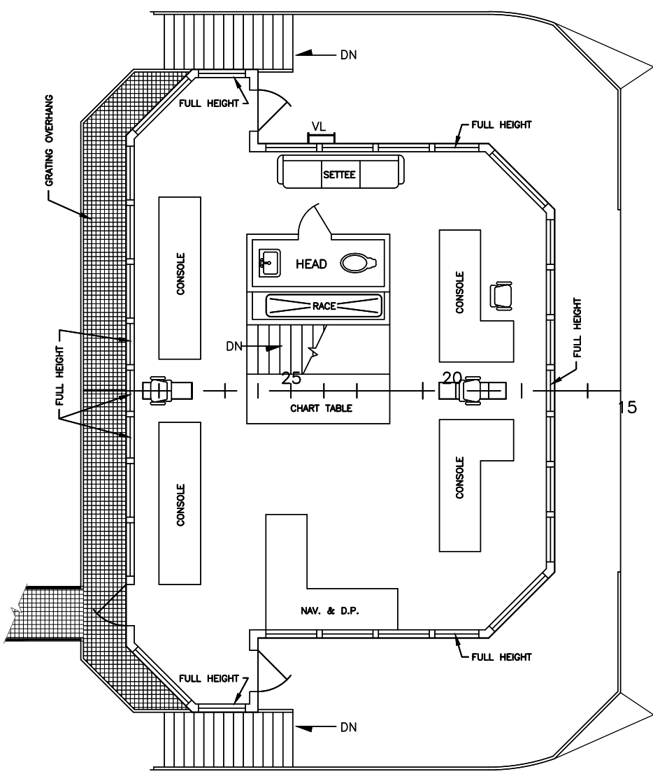
BRIDGE DECK 49'-0" ABL
